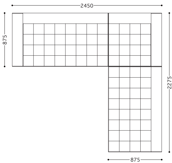
PAC-2RH1LH2S(PAC-2PR-Hi + PAC-1PL-Hi + PAC-2P-S)
